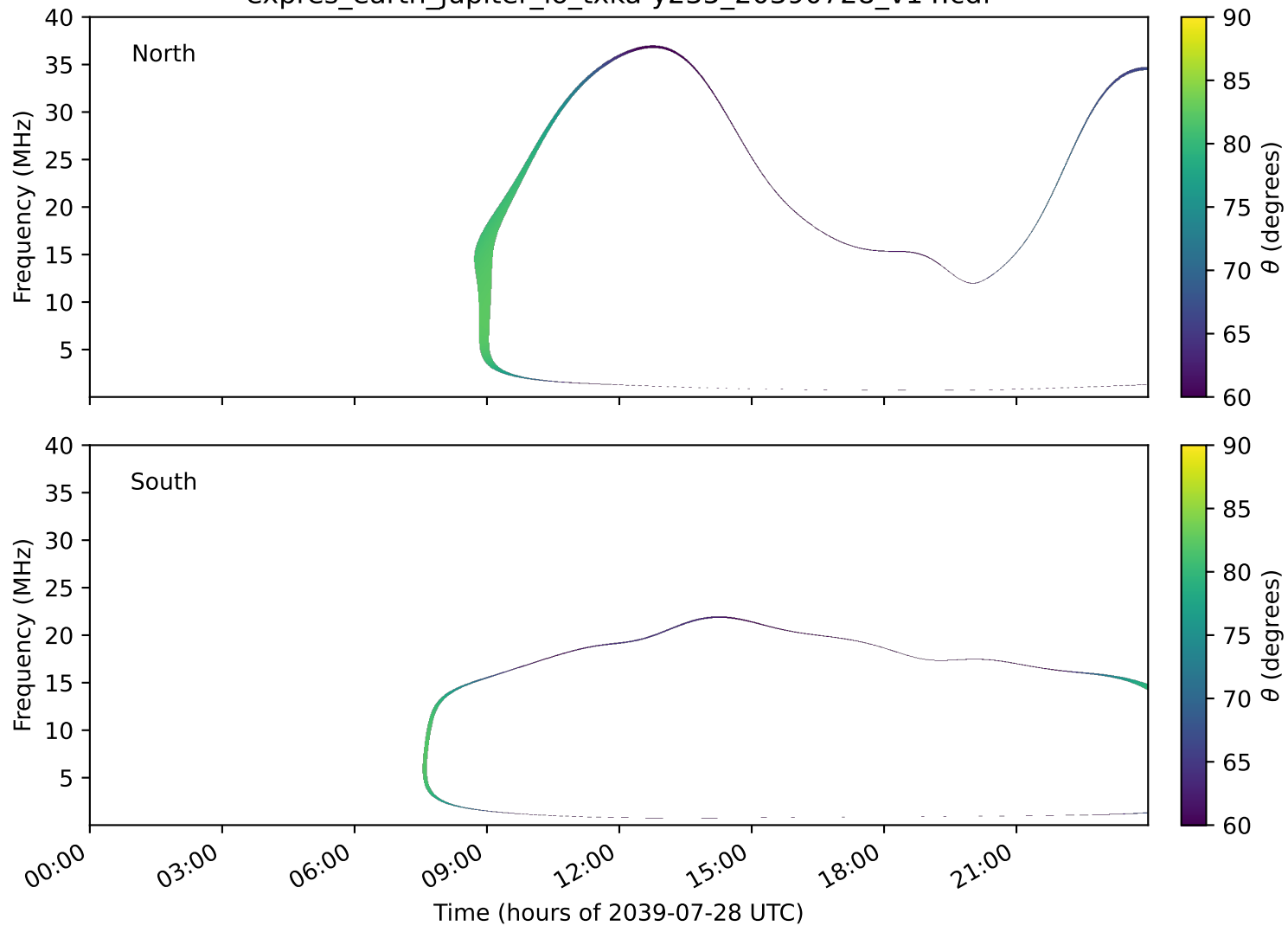
expres_earth_jupiter_io_txka-y235_20390728_v14.cdf
