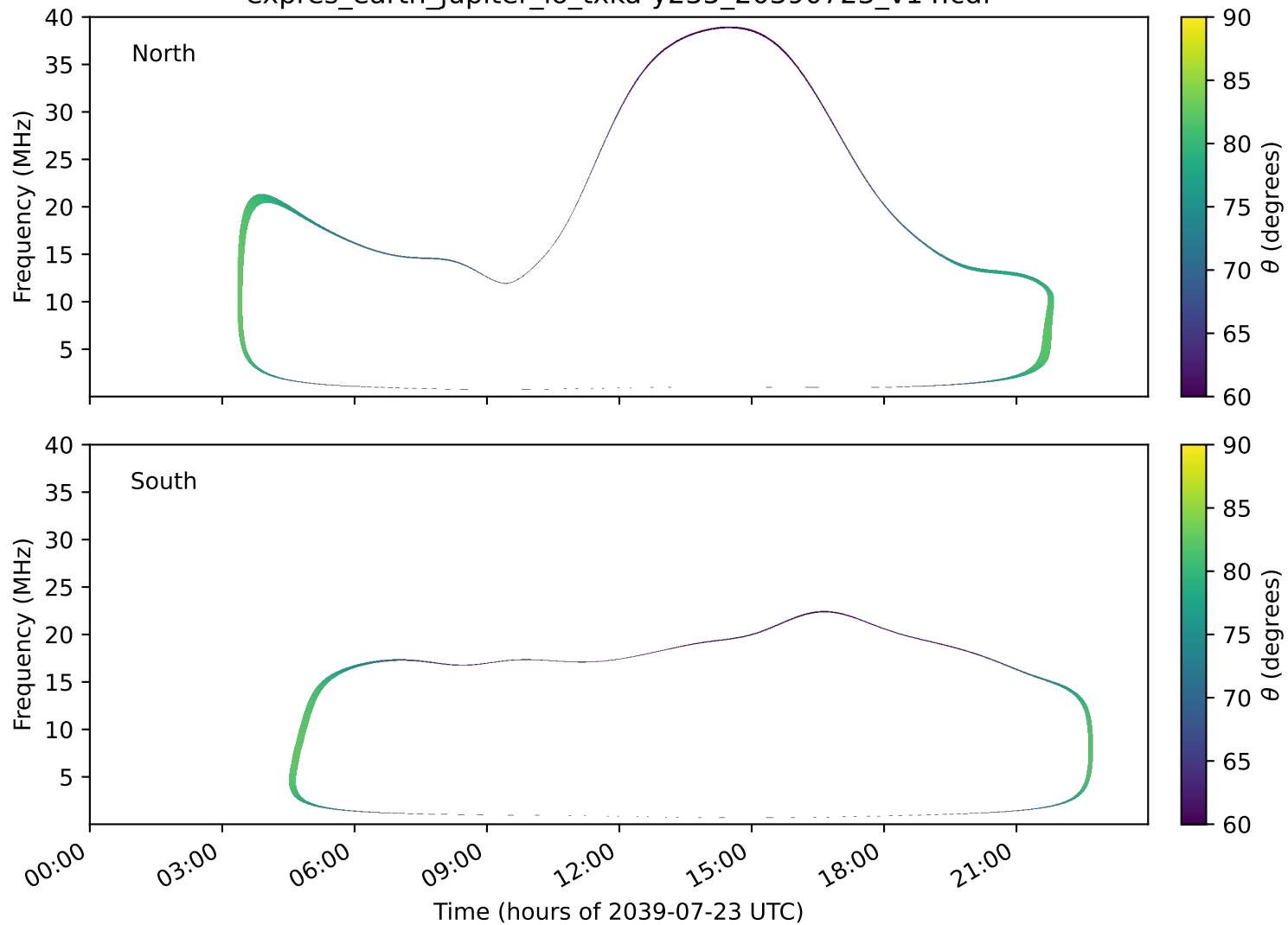
expres_earth_jupiter_io_txka-y235_20390723_v14.cdf
