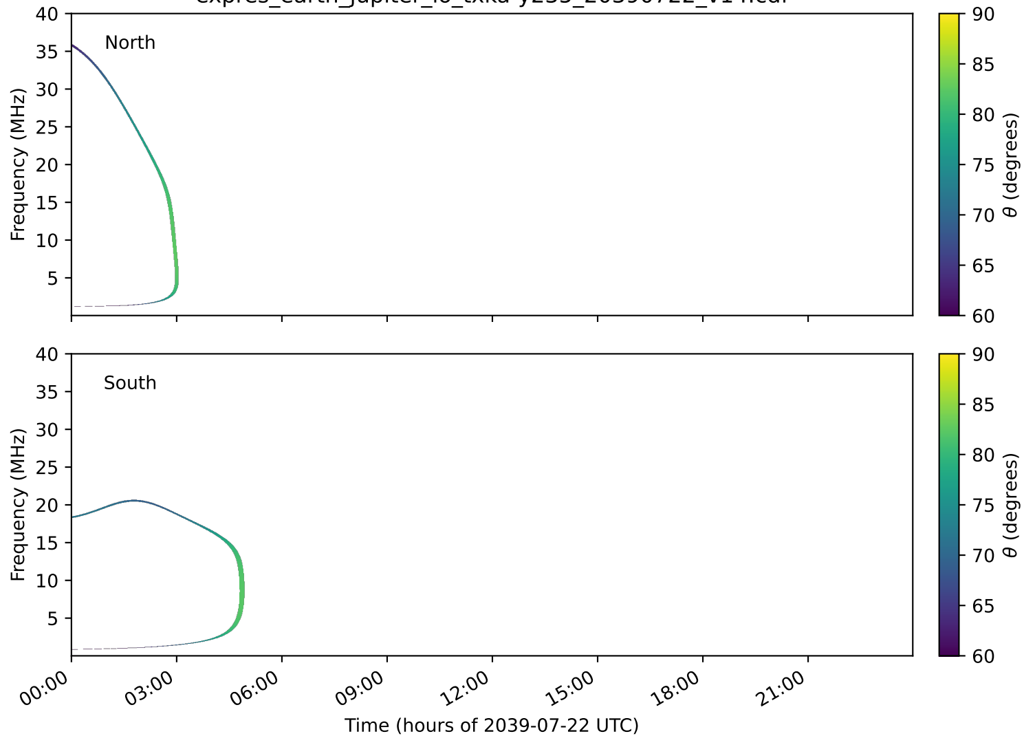
expres_earth_jupiter_io_txka-y235_20390722_v14.cdf
