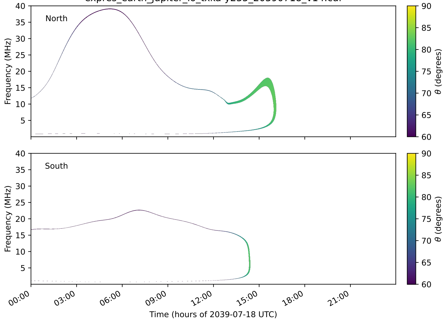
expres_earth_jupiter_io_txka-y235_20390718_v14.cdf
