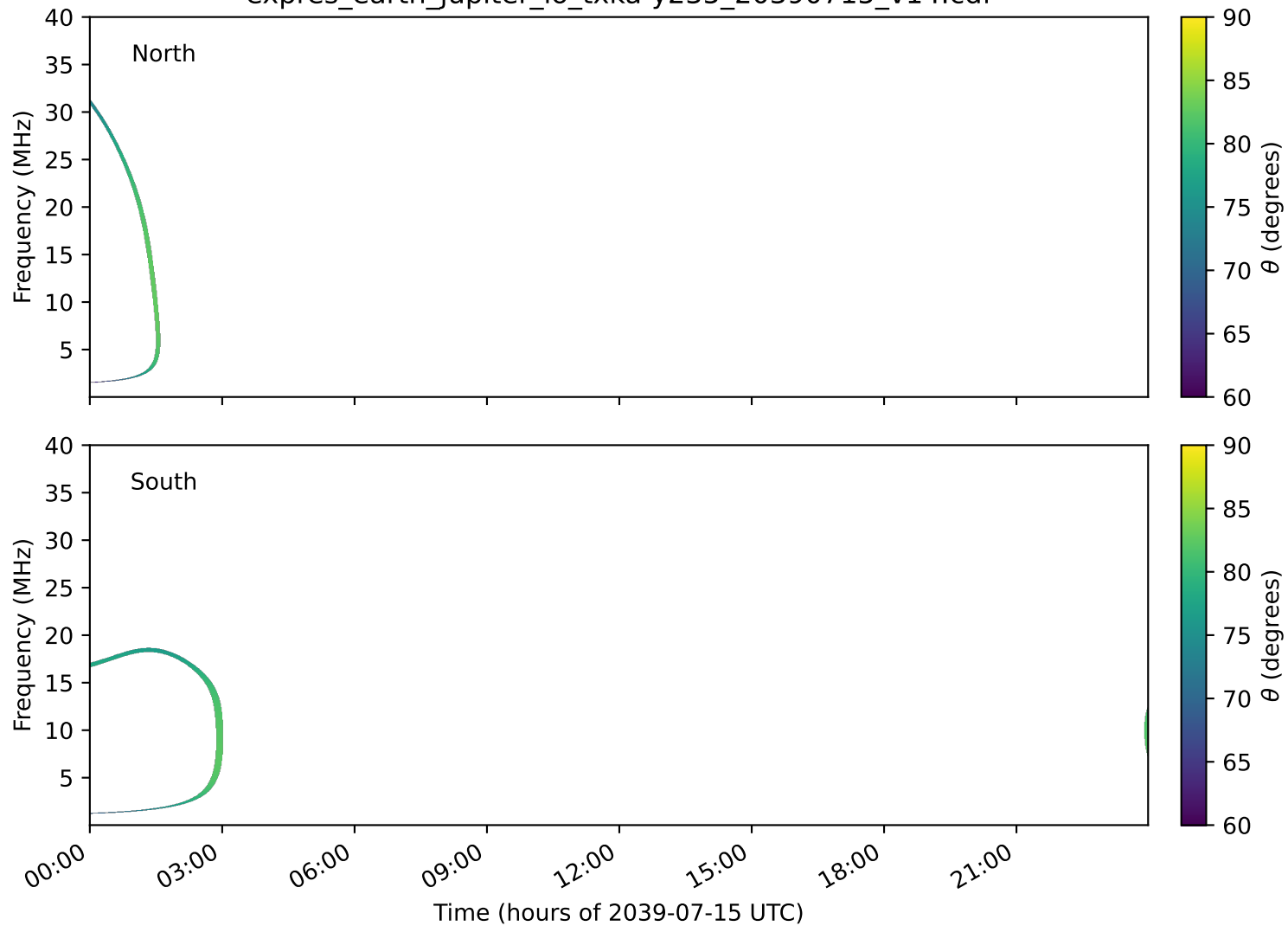
expres_earth_jupiter_io_txka-y235_20390715_v14.cdf
