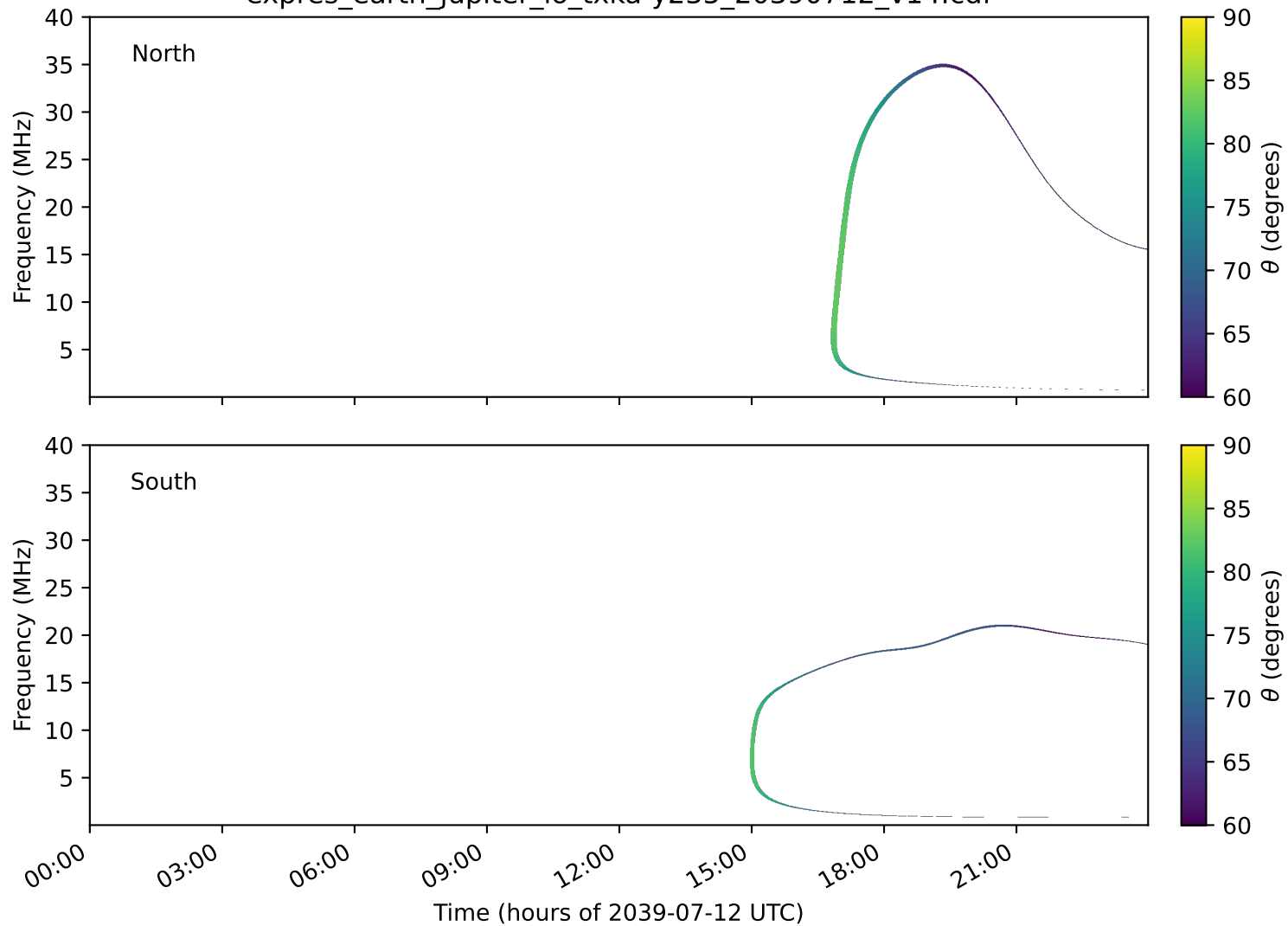
expres_earth_jupiter_io_txka-y235_20390712_v14.cdf
