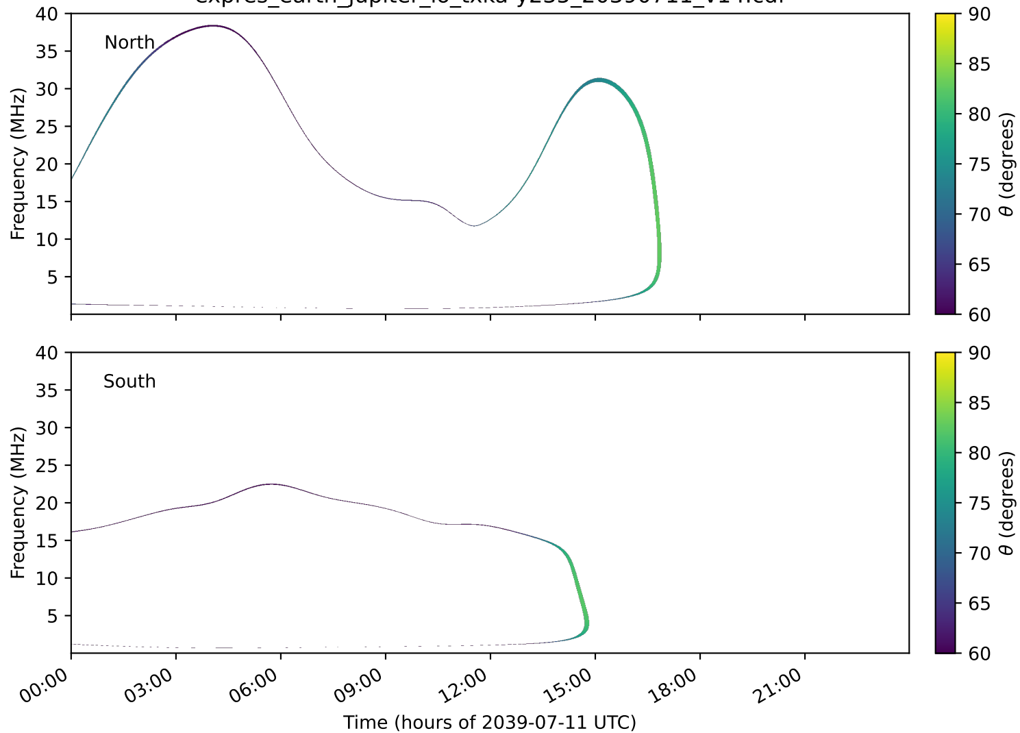
expres_earth_jupiter_io_txka-y235_20390711_v14.cdf
