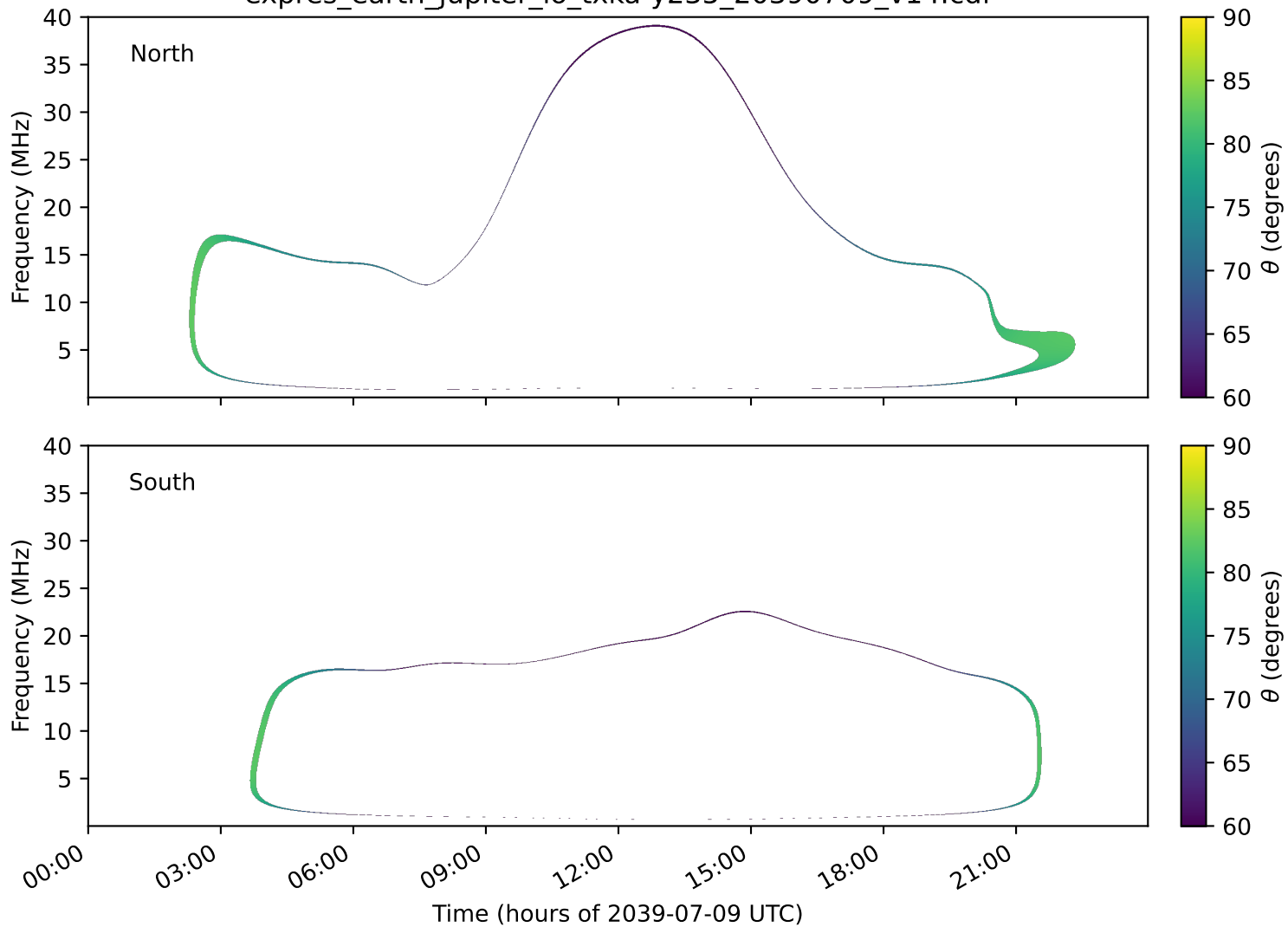
expres_earth_jupiter_io_txka-y235_20390709_v14.cdf
