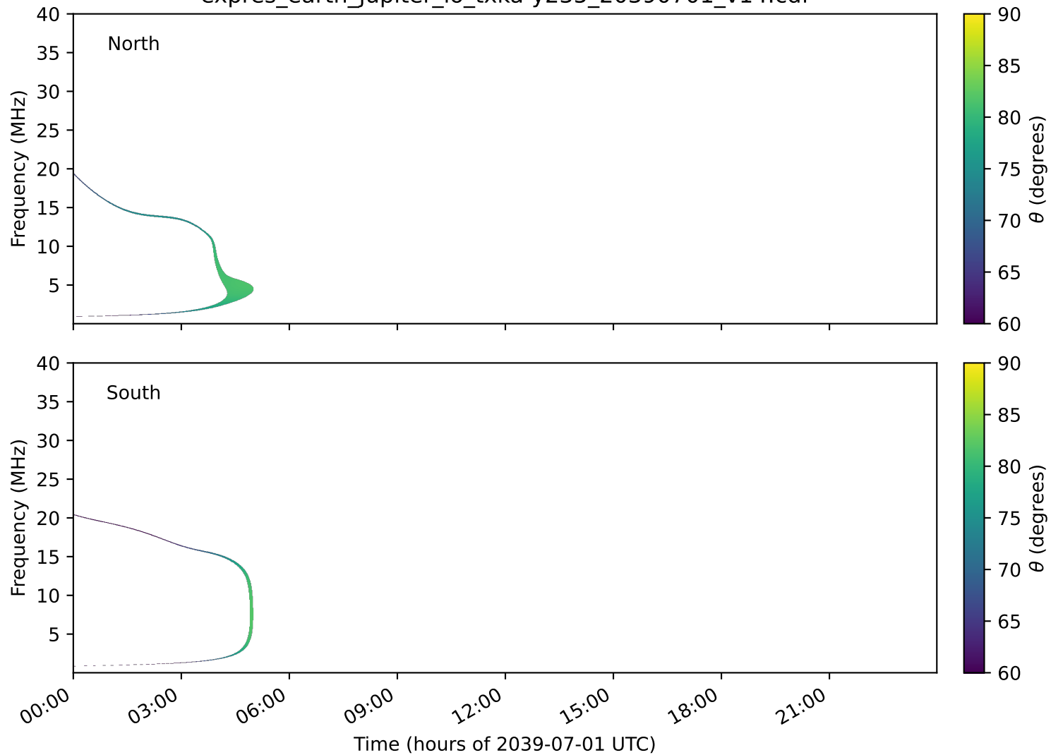
expres_earth_jupiter_io_txka-y235_20390701_v14.cdf
