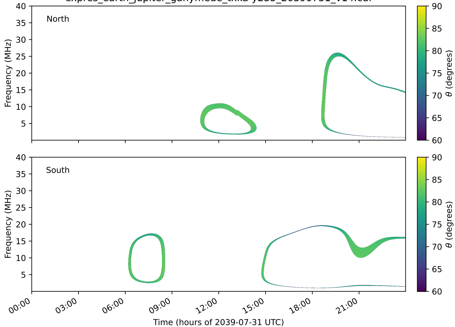
expres_earth_jupiter_ganymede_txka-y235_20390731_v14.cdf
