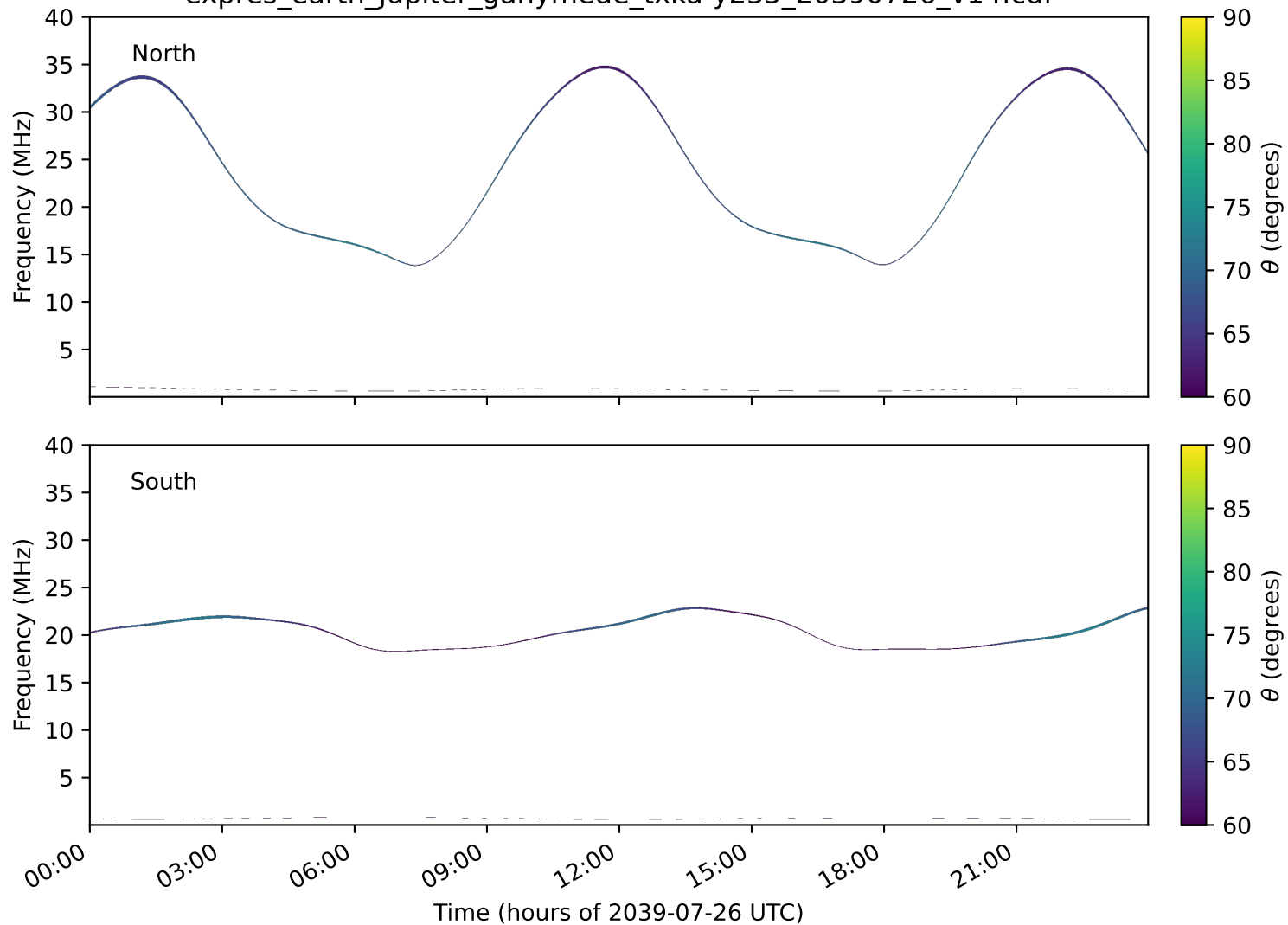
expres_earth_jupiter_ganymede_txka-y235_20390726_v14.cdf
