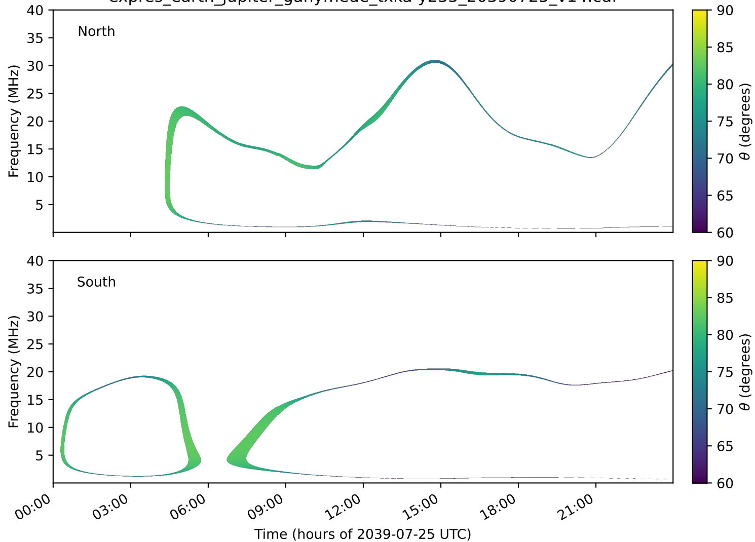
expres_earth_jupiter_ganymede_txka-y235_20390725_v14.cdf
