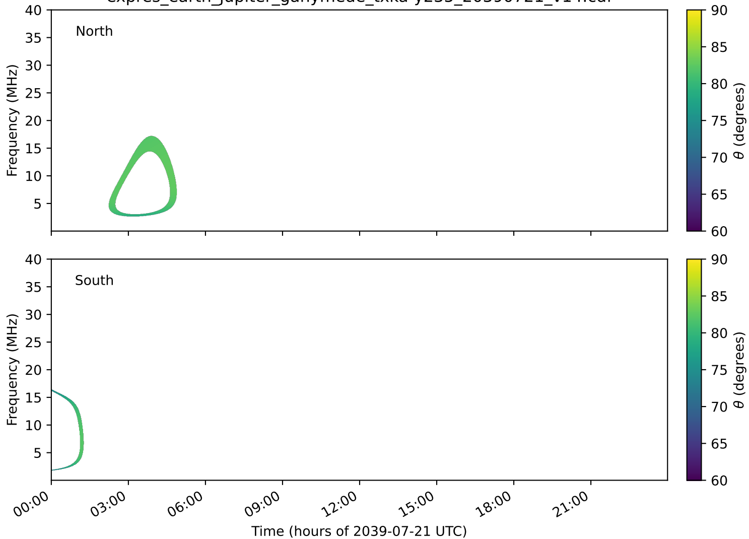
expres_earth_jupiter_ganymede_txka-y235_20390721_v14.cdf
