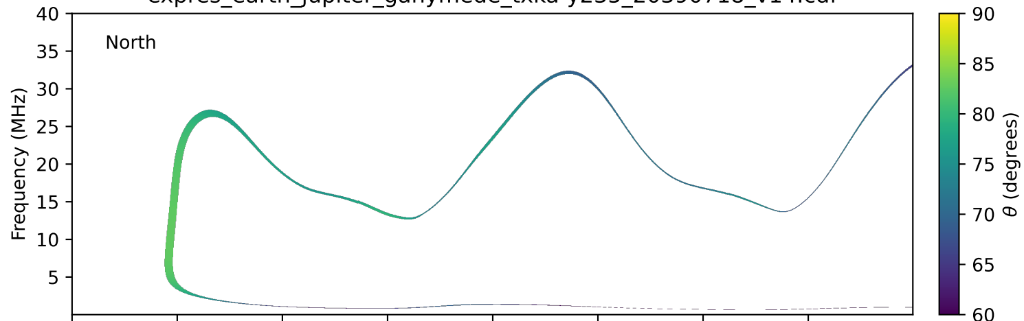
expres_earth_jupiter_ganymede_txka-y235_20390718_v14.cdf
