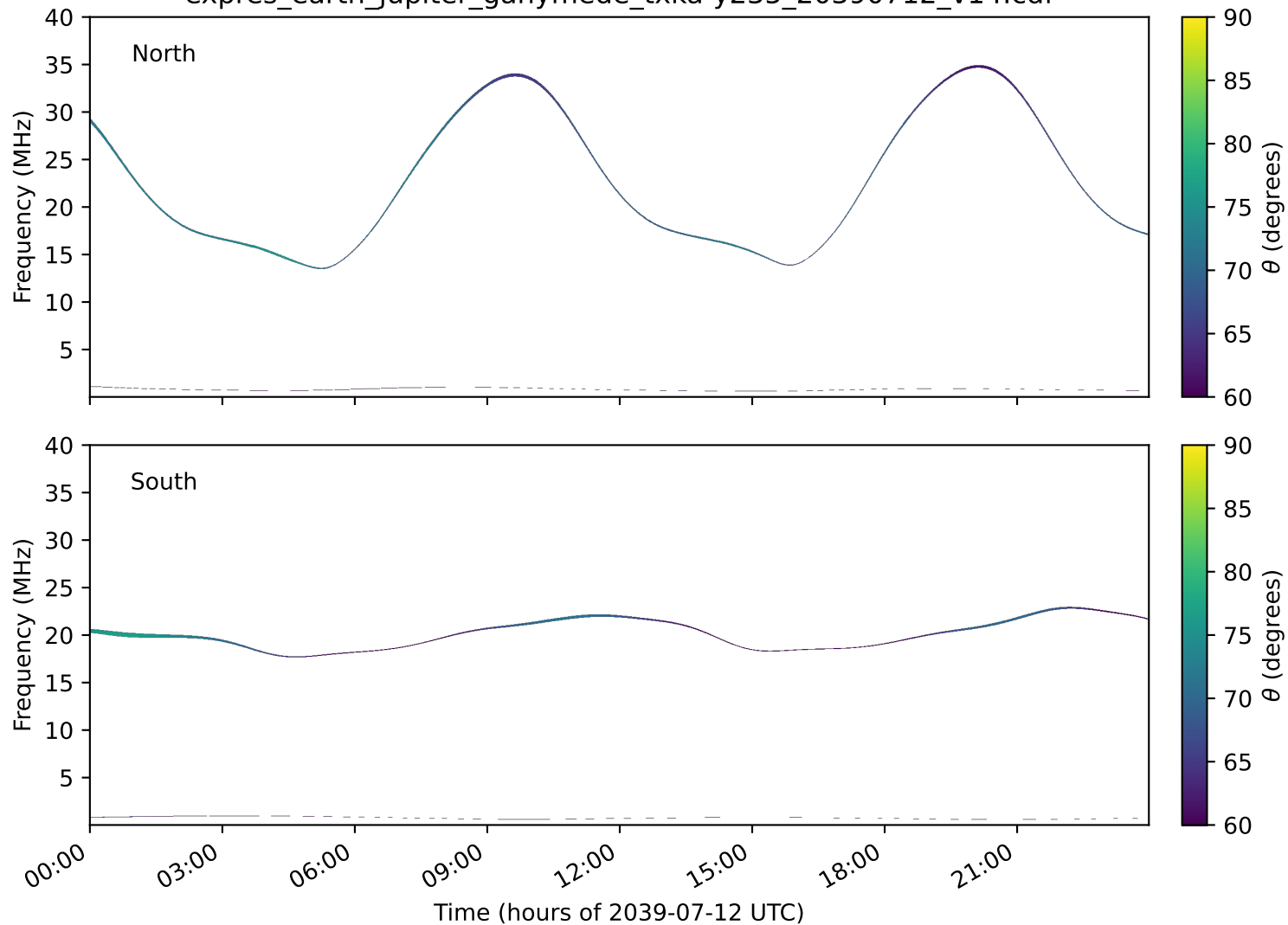
expres_earth_jupiter_ganymede_txka-y235_20390712_v14.cdf
