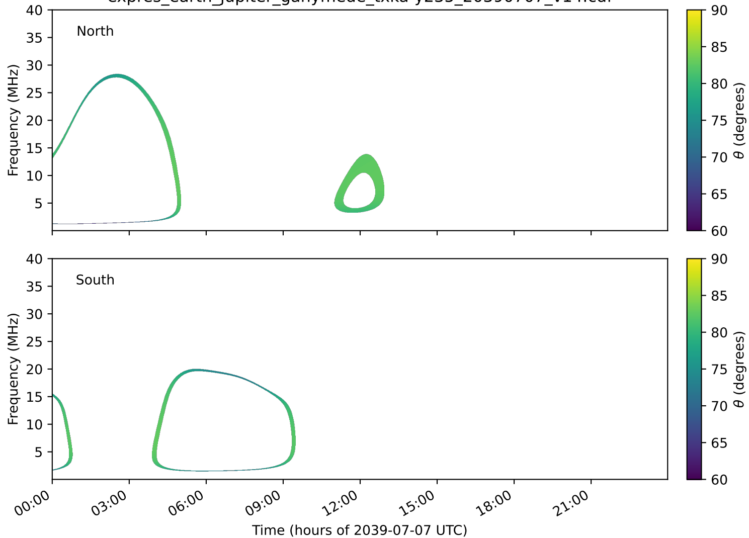
expres_earth_jupiter_ganymede_txka-y235_20390707_v14.cdf
