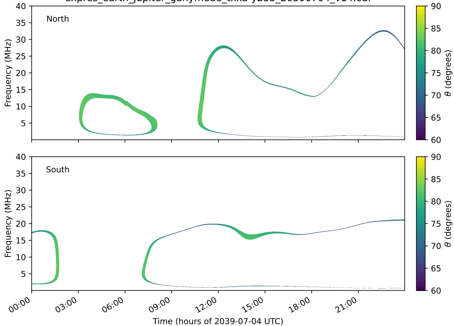
expres_earth_jupiter_ganymede_txka-y235_20390704_v14.cdf
