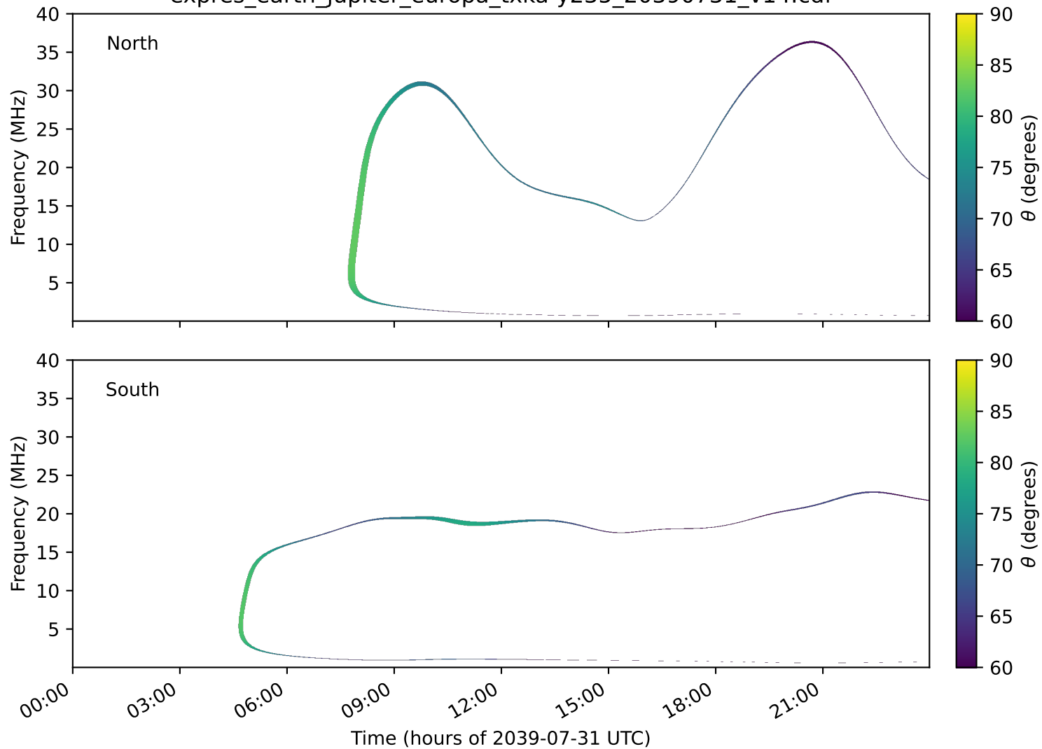
expres_earth_jupiter_europa_txka-y235_20390731_v14.cdf
