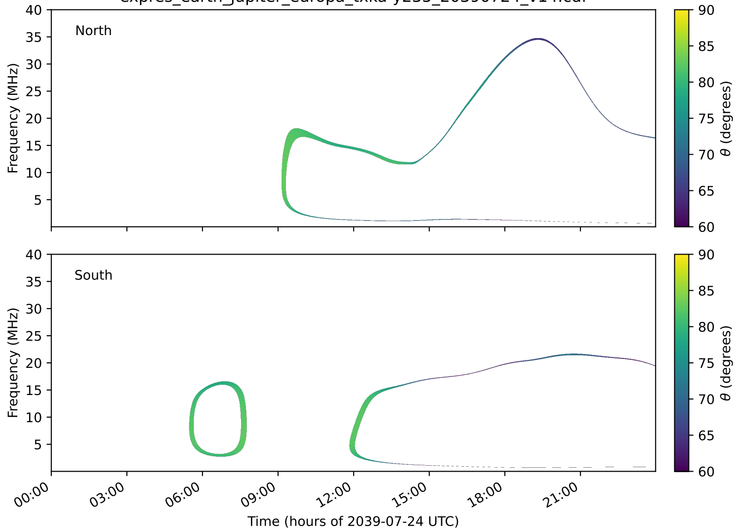
expres_earth_jupiter_europa_txka-y235_20390724_v14.cdf
