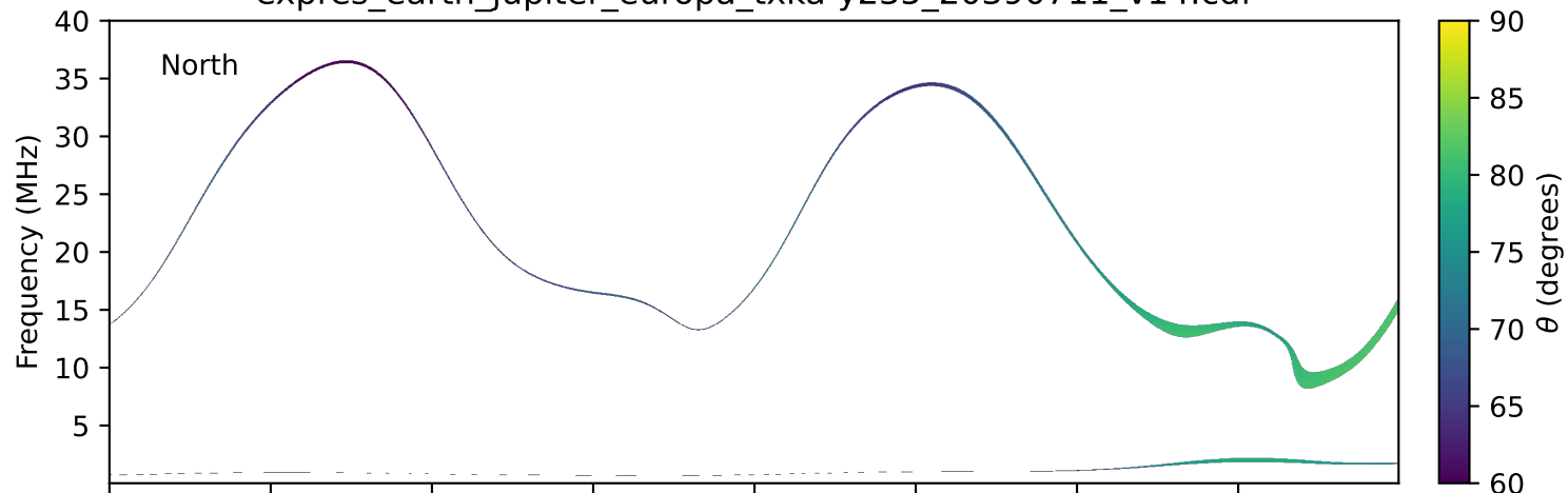
expres_earth_jupiter_europa_txka-y235_20390711_v14.cdf
