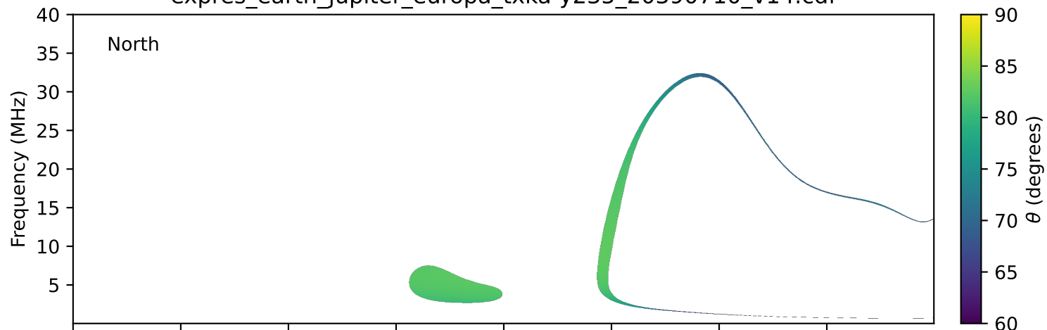
expres_earth_jupiter_europa_txka-y235_20390710_v14.cdf
