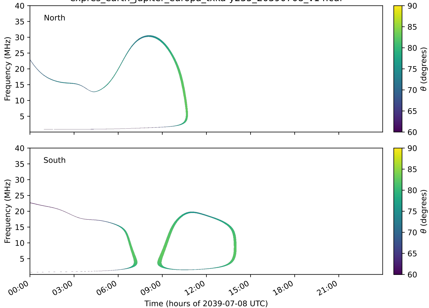
expres_earth_jupiter_europa_txka-y235_20390708_v14.cdf
