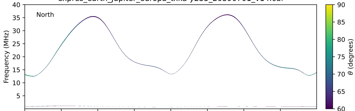
expres_earth_jupiter_europa_txka-y235_20390701_v14.cdf
