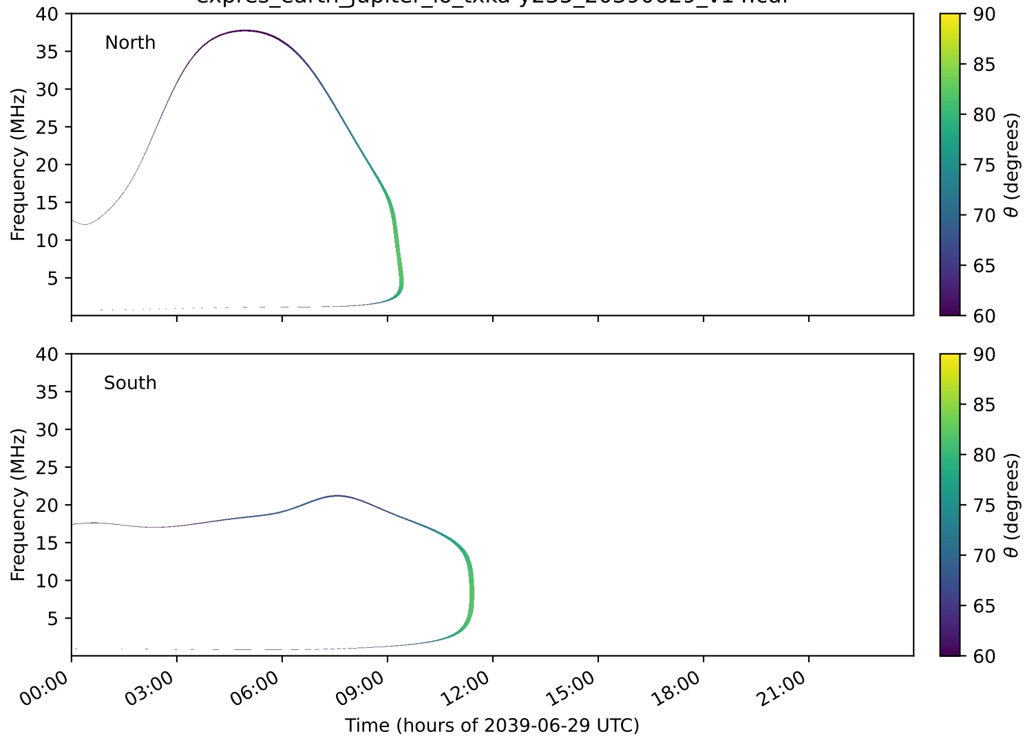
expres_earth_jupiter_io_txka-y235_20390629_v14.cdf
