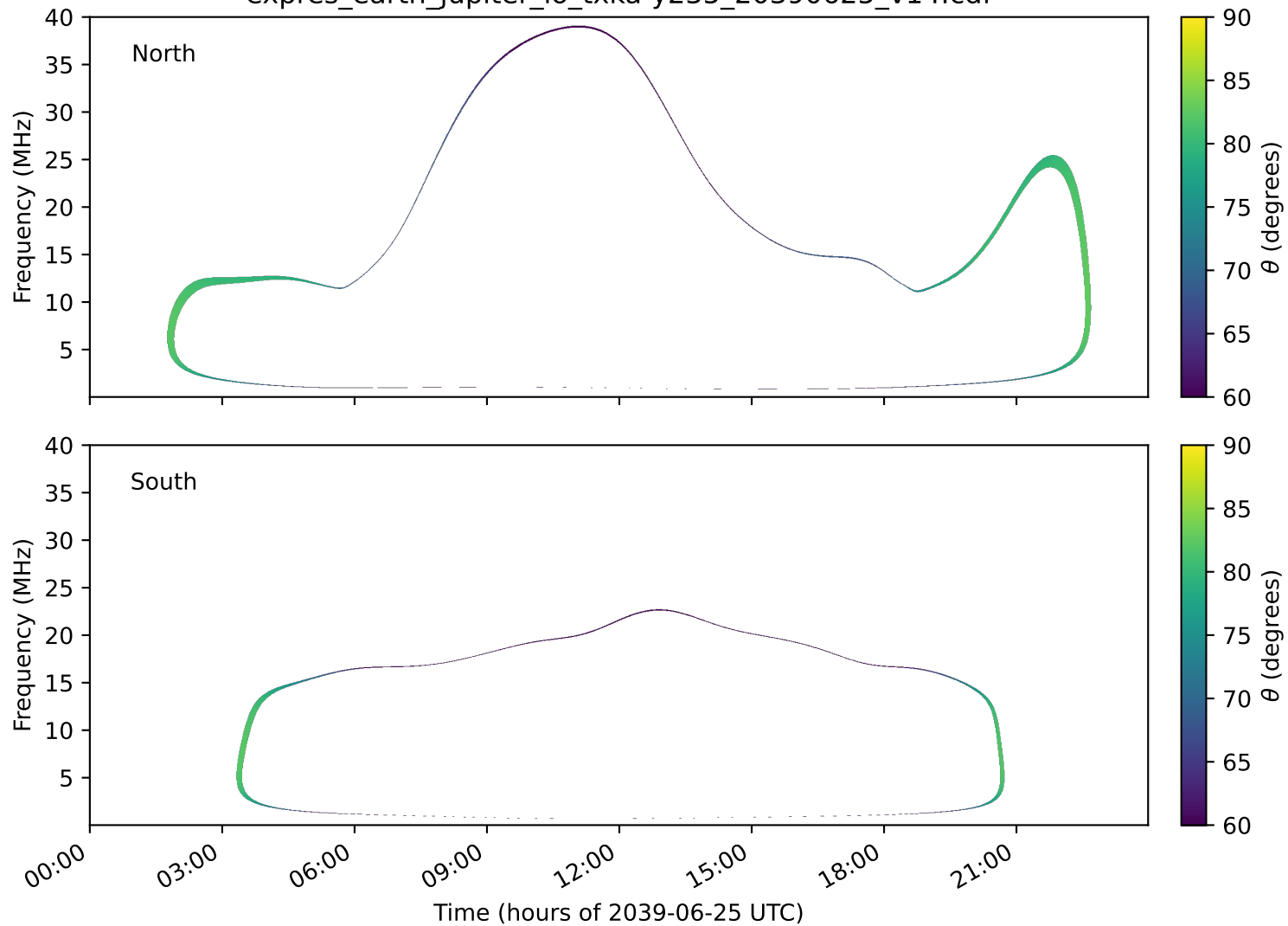
expres_earth_jupiter_io_txka-y235_20390625_v14.cdf
