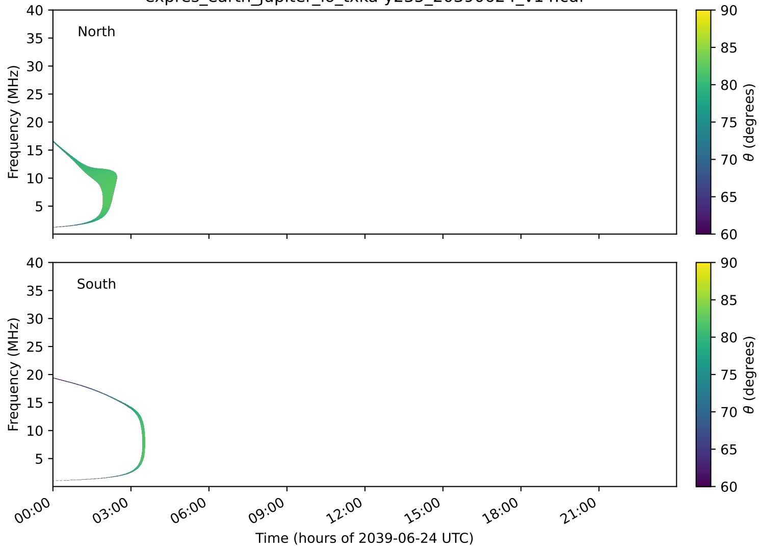
expres_earth_jupiter_io_txka-y235_20390624_v14.cdf
