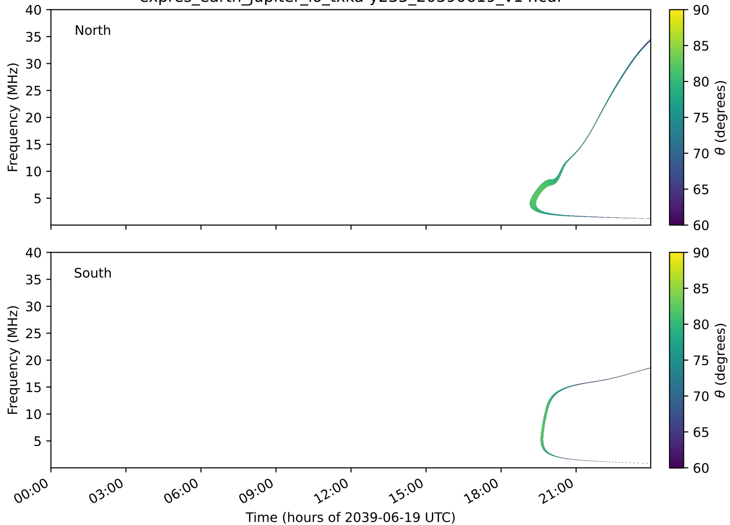
expres_earth_jupiter_io_txka-y235_20390619_v14.cdf
