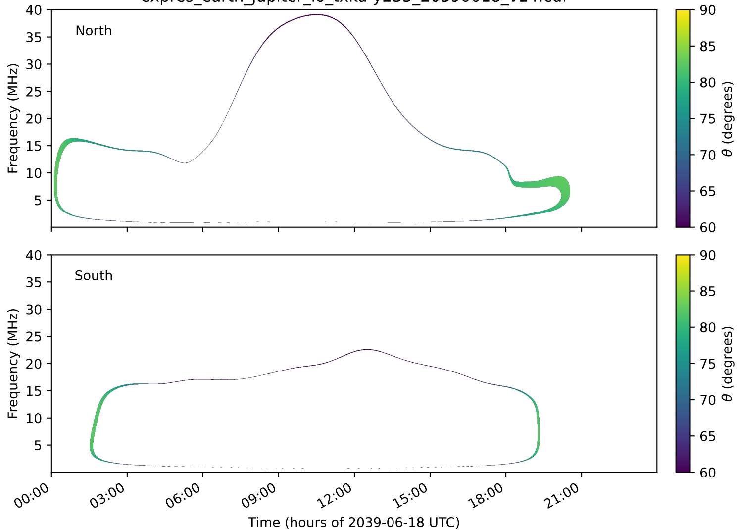
expres_earth_jupiter_io_txka-y235_20390618_v14.cdf
