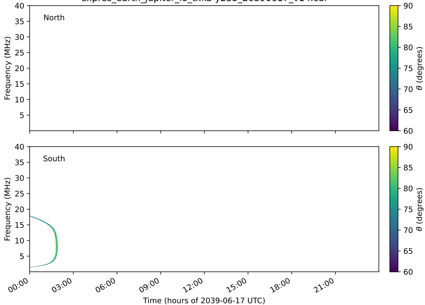
expres_earth_jupiter_io_txka-y235_20390617_v14.cdf
