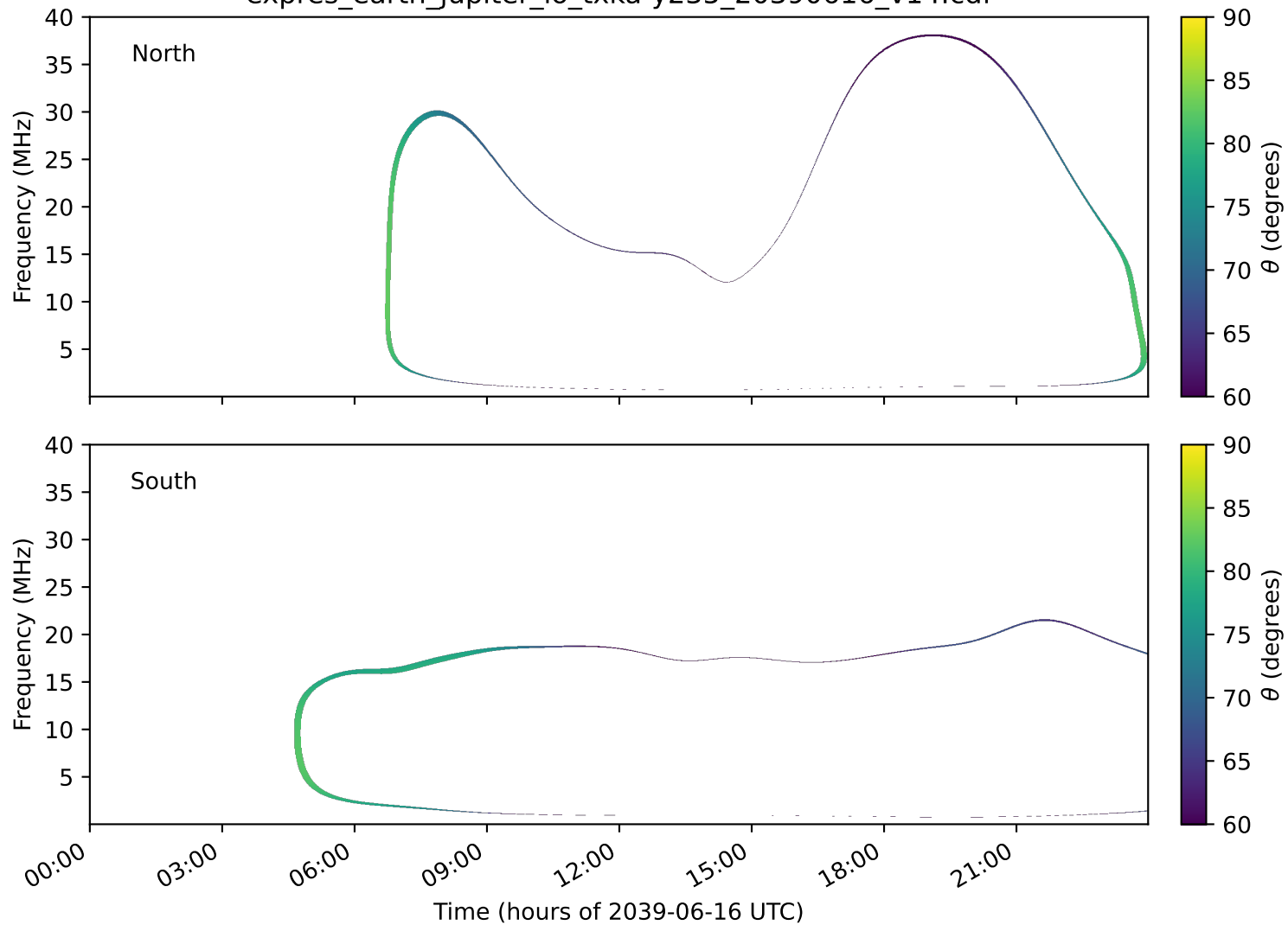
expres_earth_jupiter_io_txka-y235_20390616_v14.cdf
