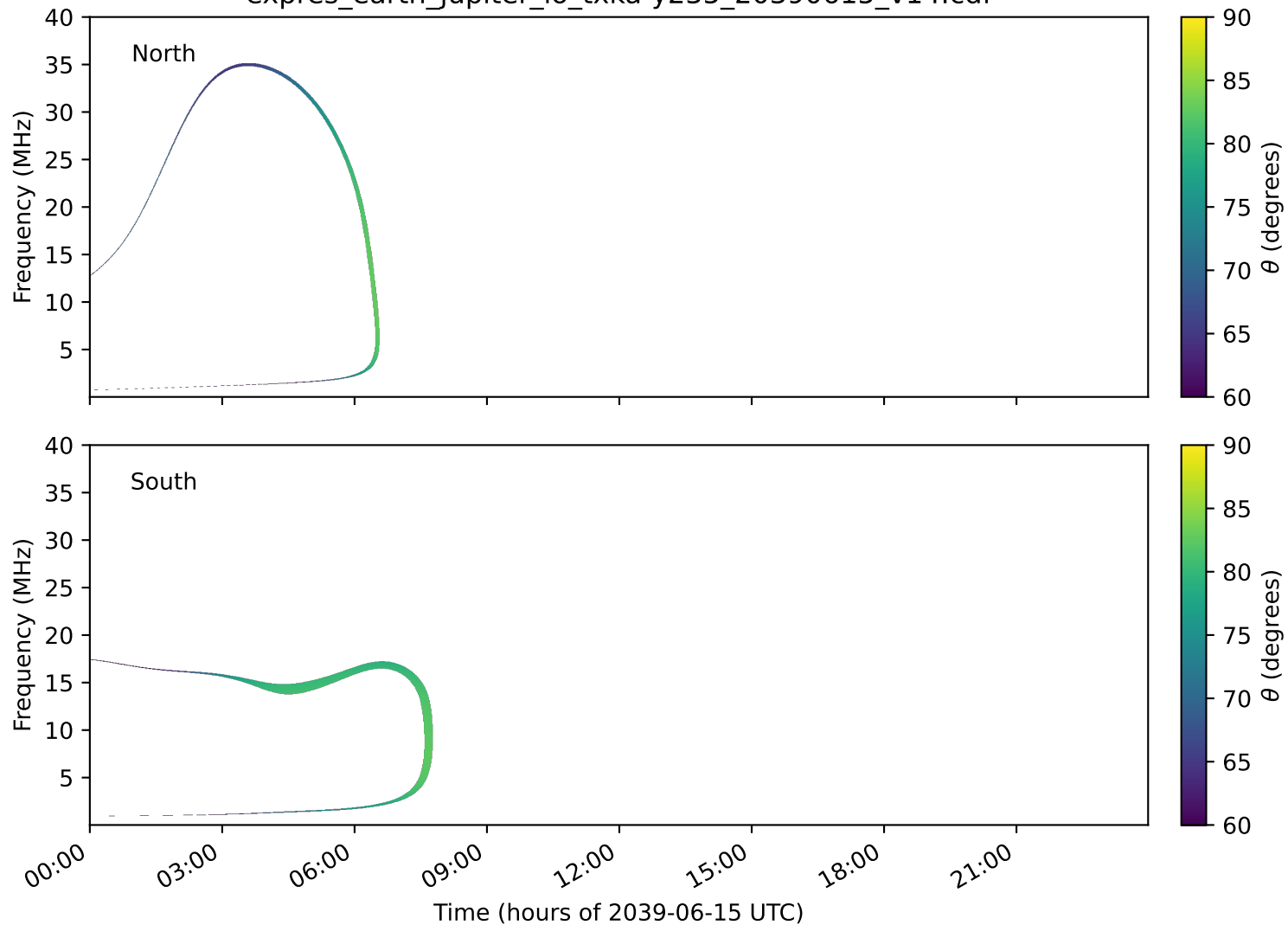
expres_earth_jupiter_io_txka-y235_20390615_v14.cdf
