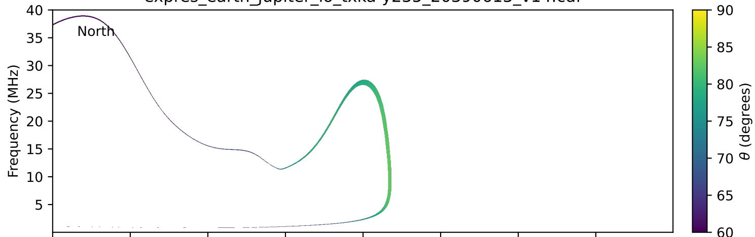
expres_earth_jupiter_io_txka-y235_20390613_v14.cdf
