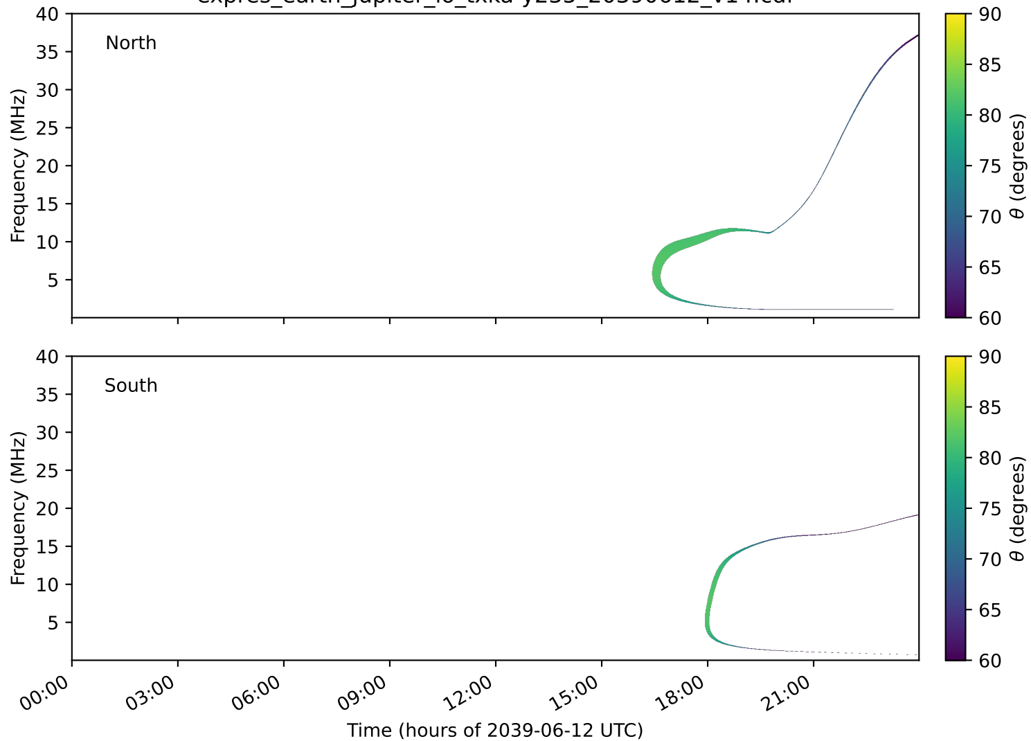
expres_earth_jupiter_io_txka-y235_20390612_v14.cdf
