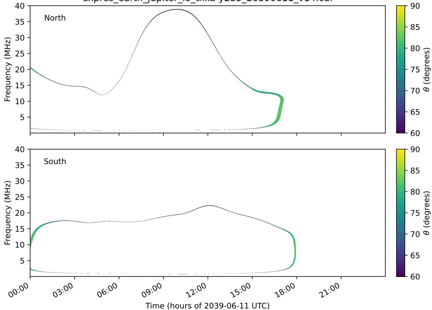
expres_earth_jupiter_io_txka-y235_20390611_v14.cdf
