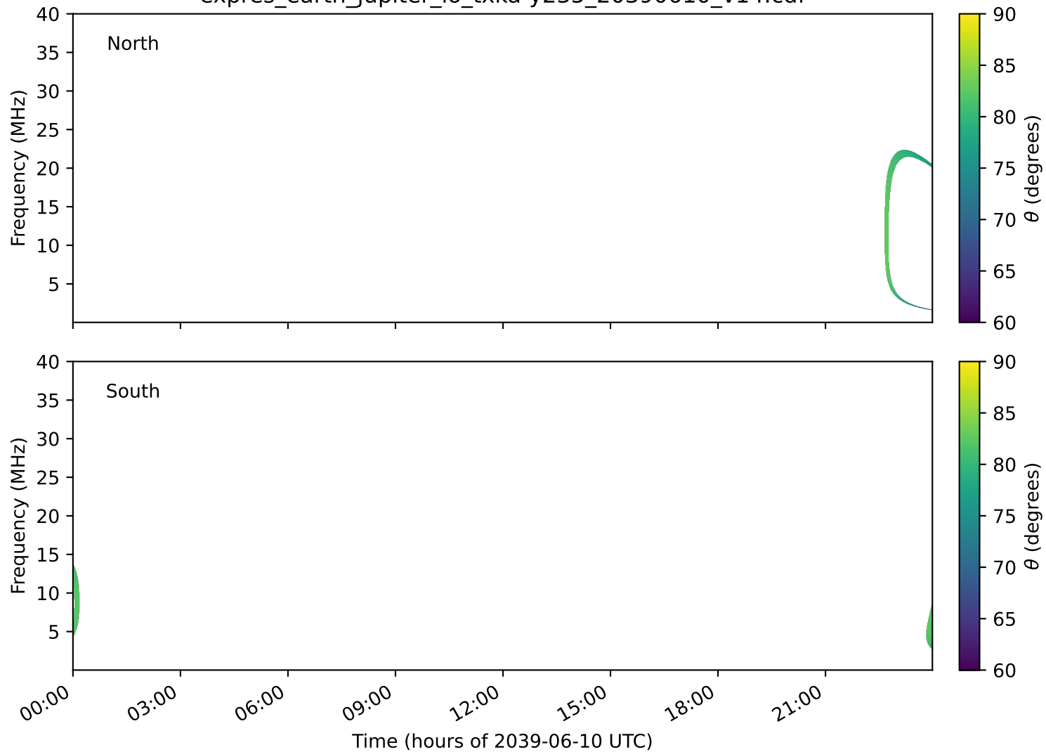
expres_earth_jupiter_io_txka-y235_20390610_v14.cdf
