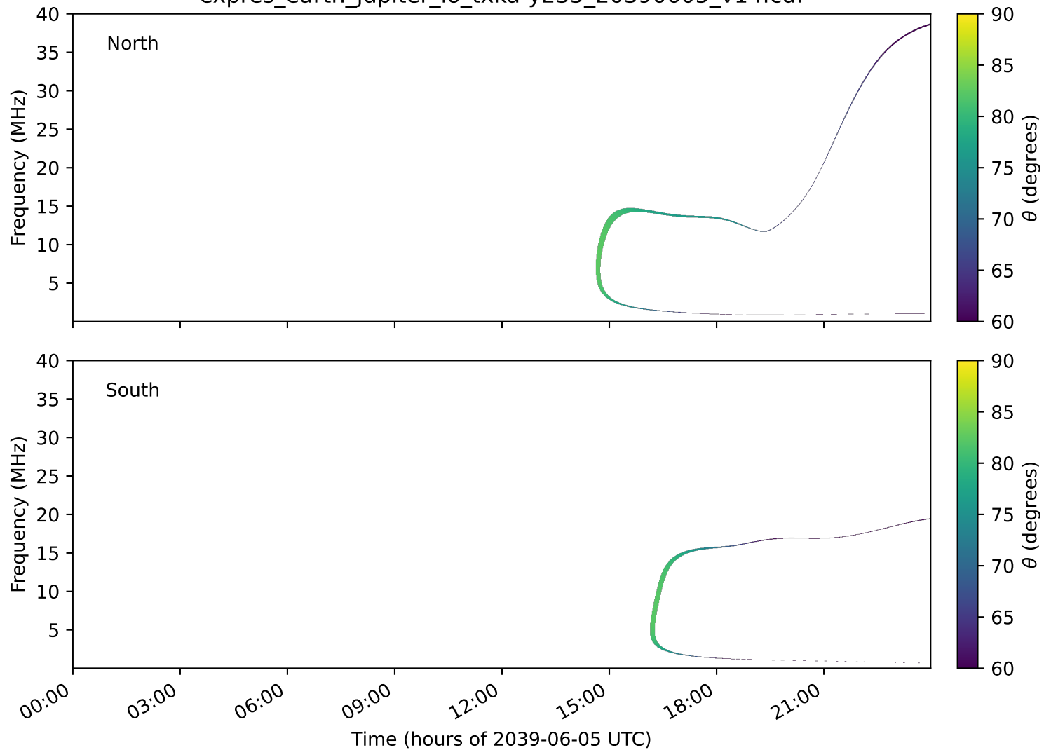
expres_earth_jupiter_io_txka-y235_20390605_v14.cdf
