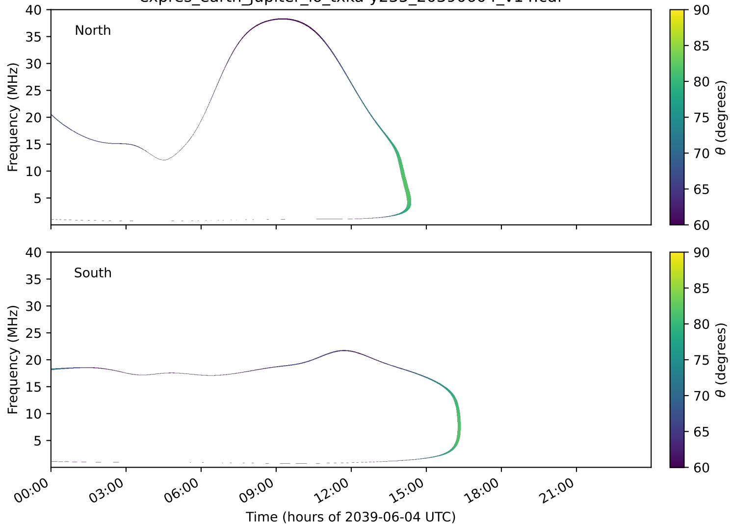
expres_earth_jupiter_io_txka-y235_20390604_v14.cdf
