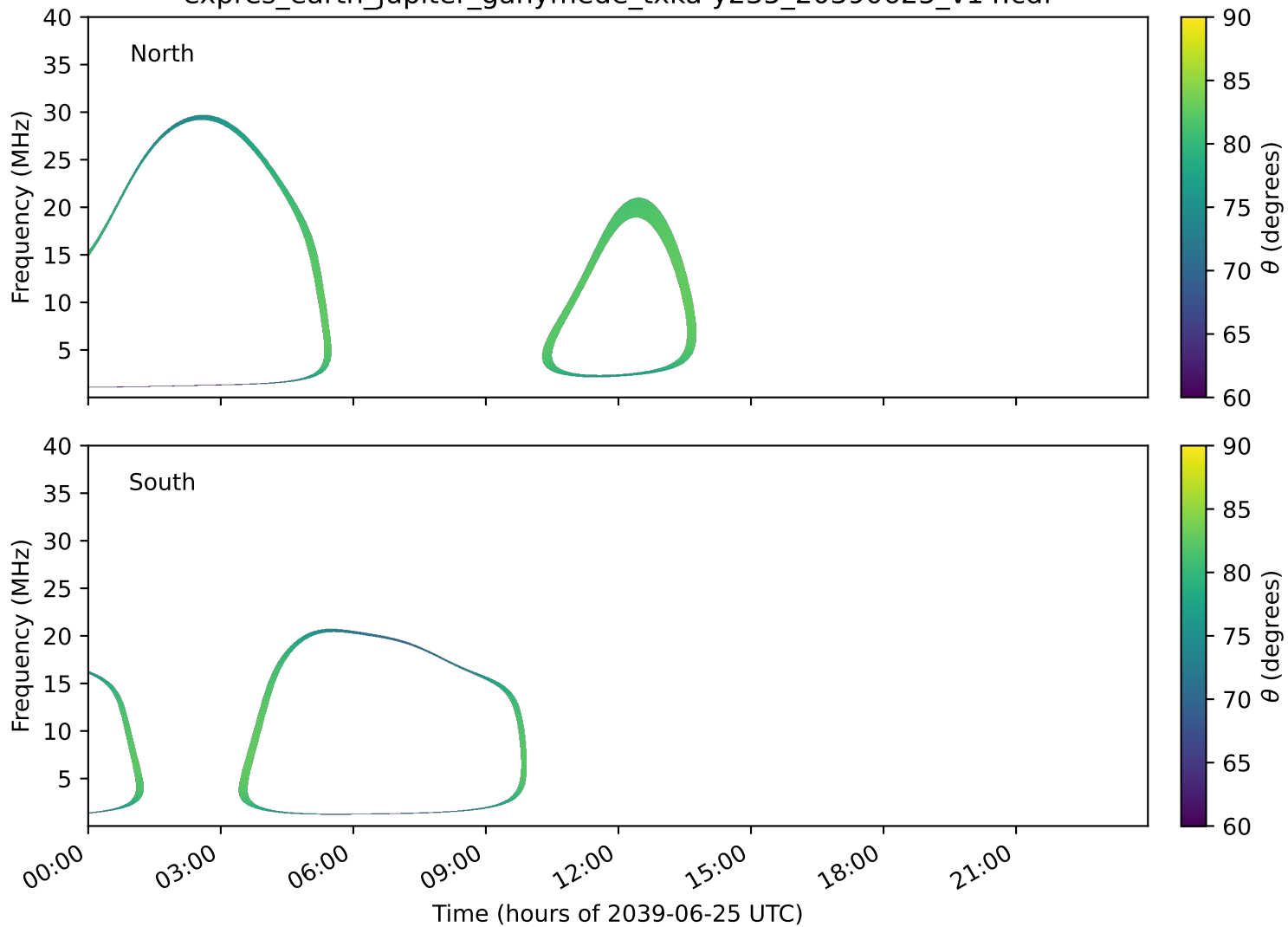
expres_earth_jupiter_ganymede_txka-y235_20390625_v14.cdf
