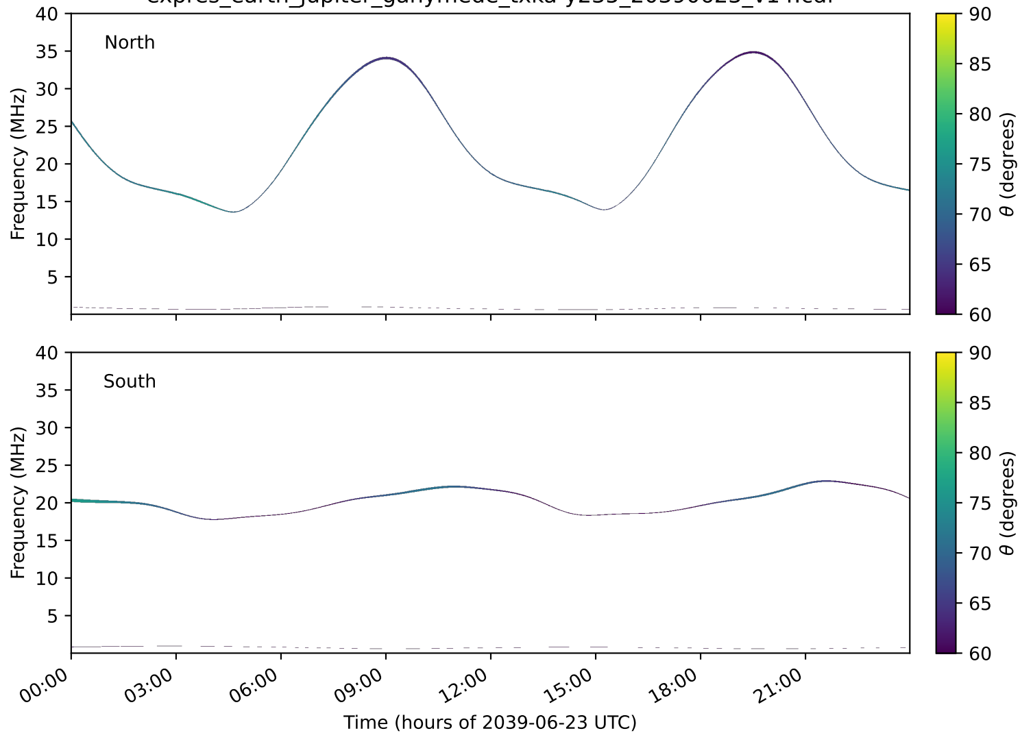
expres_earth_jupiter_ganymede_txka-y235_20390623_v14.cdf
