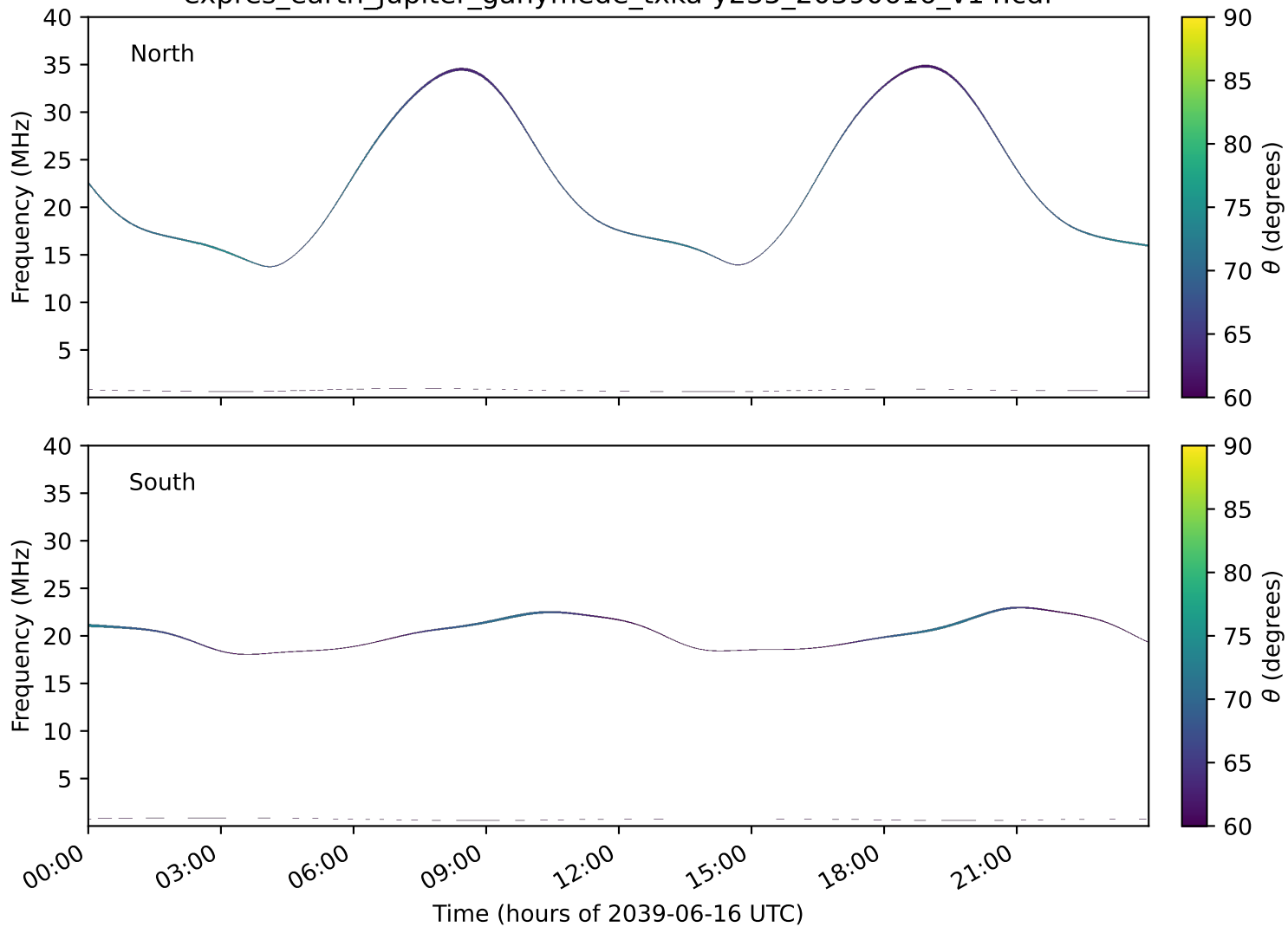
expres_earth_jupiter_ganymede_txka-y235_20390616_v14.cdf
