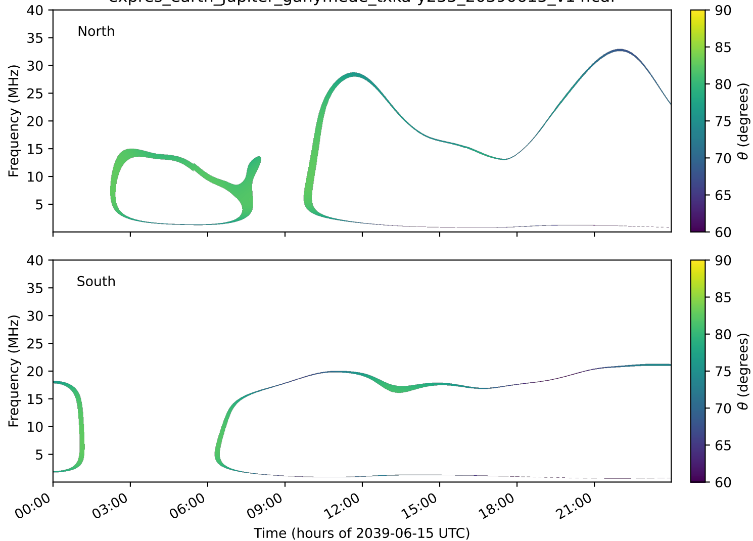
expres_earth_jupiter_ganymede_txka-y235_20390615_v14.cdf
