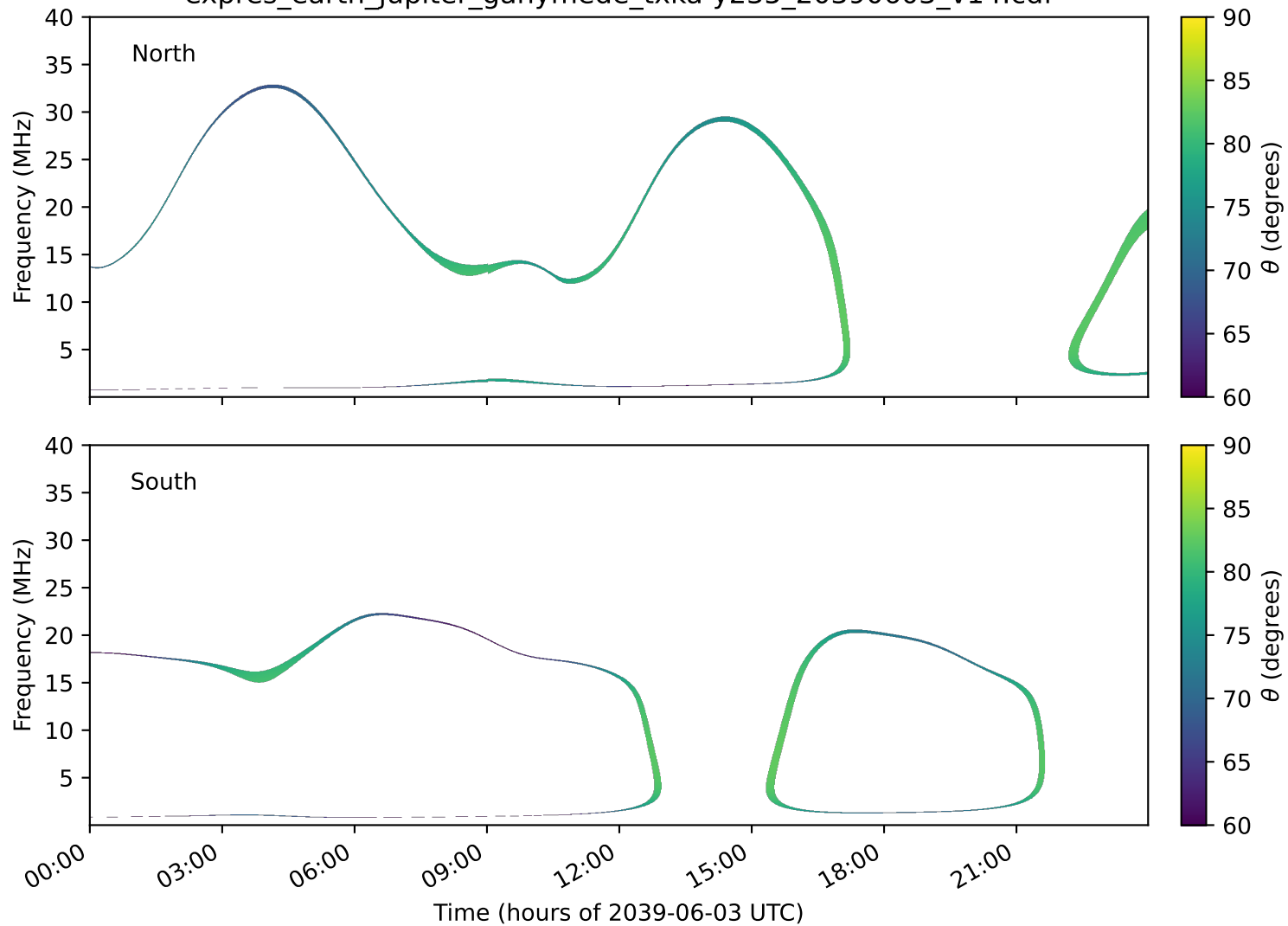
expres_earth_jupiter_ganymede_txka-y235_20390603_v14.cdf
