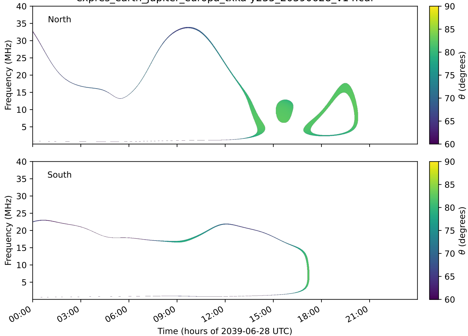
expres_earth_jupiter_europa_txka-y235_20390628_v14.cdf
