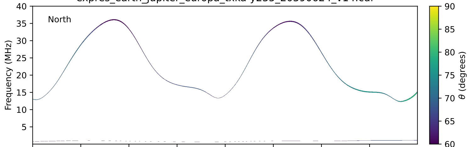
expres_earth_jupiter_europa_txka-y235_20390624_v14.cdf
