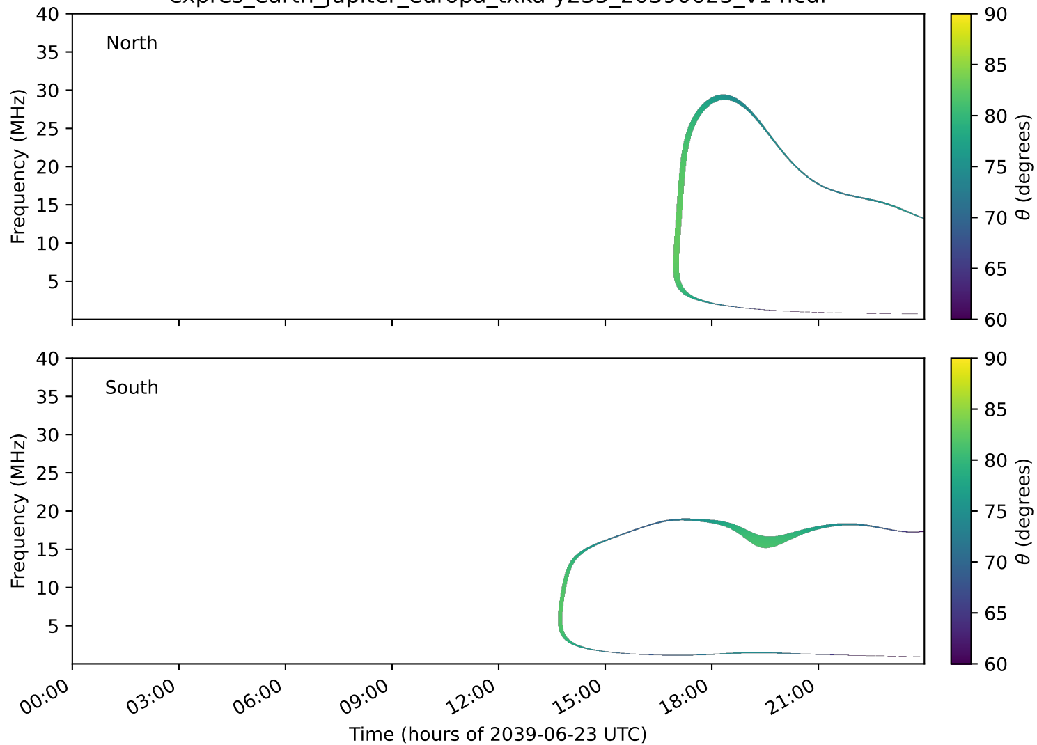
expres_earth_jupiter_europa_txka-y235_20390623_v14.cdf
