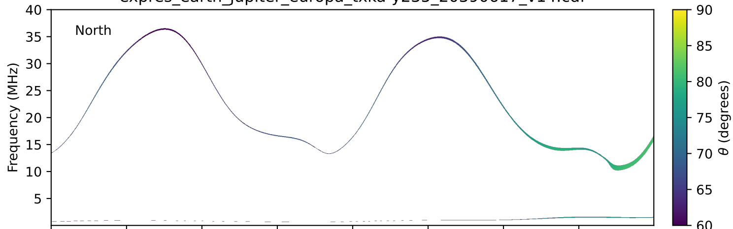
expres_earth_jupiter_europa_txka-y235_20390617_v14.cdf
