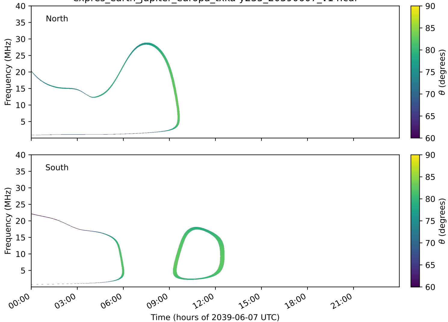
expres_earth_jupiter_europa_txka-y235_20390607_v14.cdf
