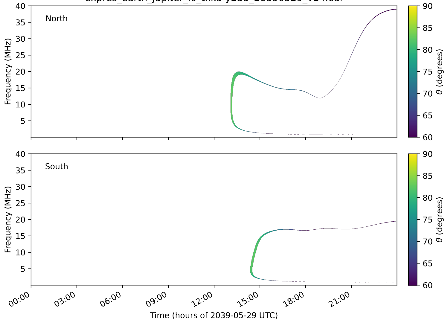
expres_earth_jupiter_io_txka-y235_20390529_v14.cdf
