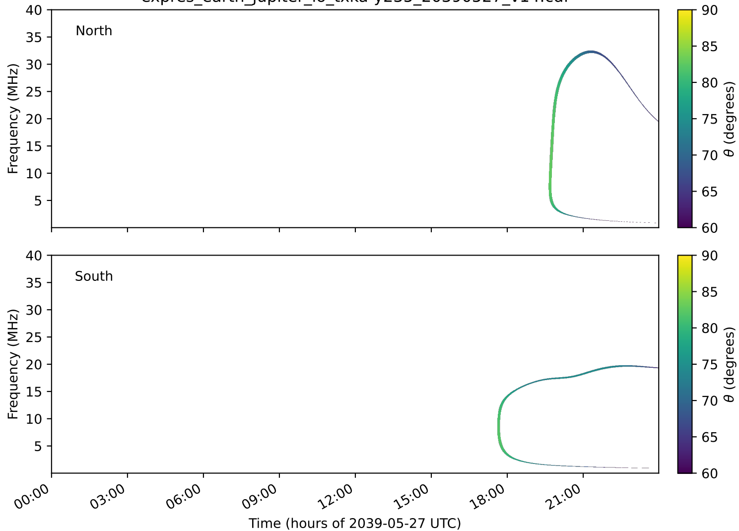
expres_earth_jupiter_io_txka-y235_20390527_v14.cdf
