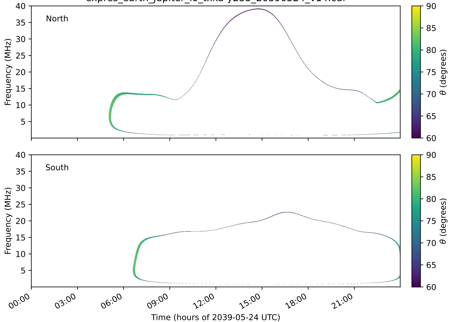
expres_earth_jupiter_io_txka-y235_20390524_v14.cdf
